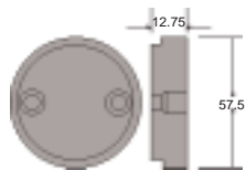
FTL 153 PK Unlined steel Piston with Screws & Washers
